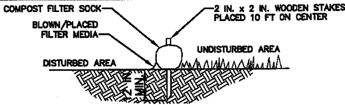
SECTION
