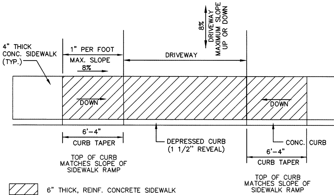
PLAN OF 4' SIDEWALK ADJACENT TO CURB
