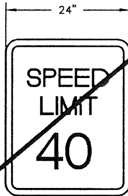
R2-1, 24"X30" SPEED LIMIT SIGN
