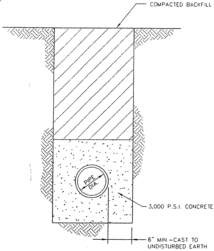
SECTION
