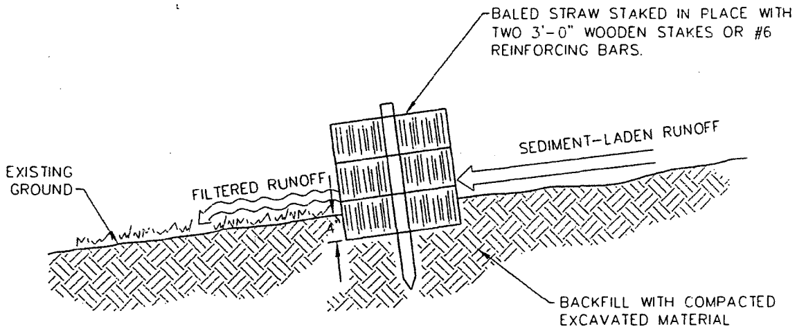
CROSS-SECTION OF PROPERLY INSTALLED STRAW BALE
