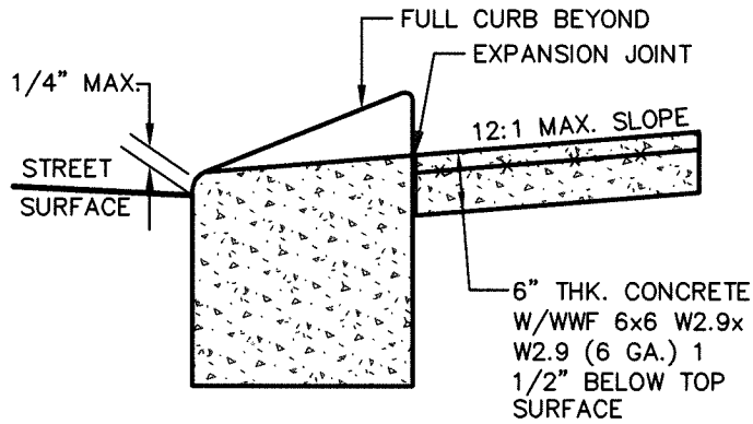
CROSS SECTION AT HANDICAP RAMPS
