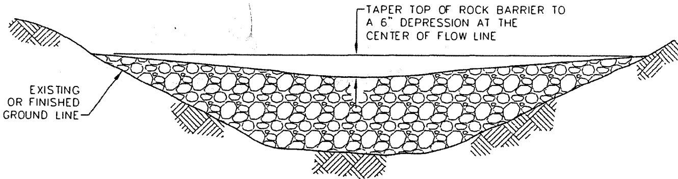
SECTION B-B
